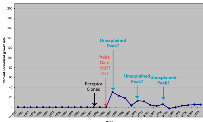
SF1 Normalized growth rates 1980-2010
