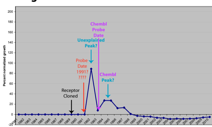
RARg Normalized growth rates 1980-2010
