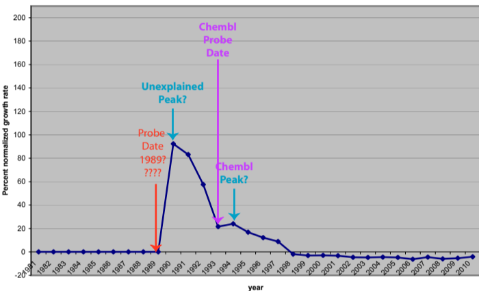
RXRb Normalized Growth Rate 1980-2010
