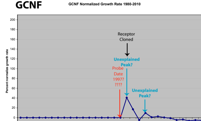
GCNF Normalized Growth Rate 1980-2010
