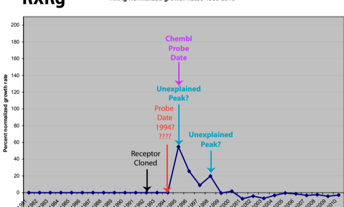
RXRg Normalized growth Rates 1980-2010
