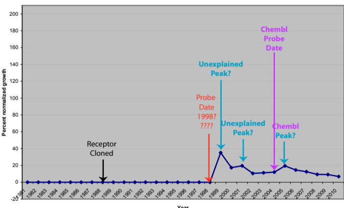
ERRa Normalized Growth Rates (1980-2010)
