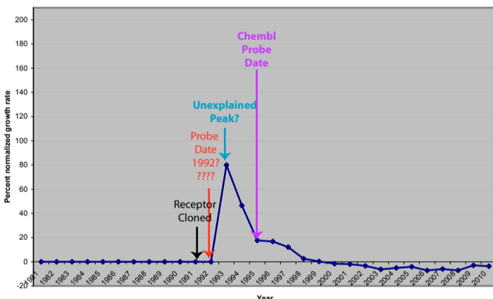
Rev-erbB Normalized Growth Rate 1980-2010
